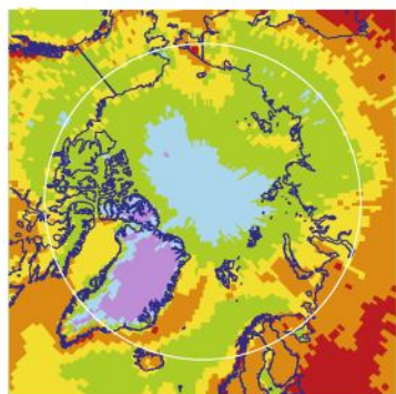
GRAHM model
