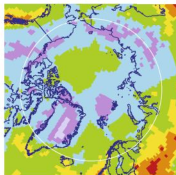
DEHM model
