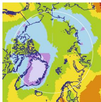
GLEMOS model
