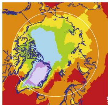
GEOS-Chem model
